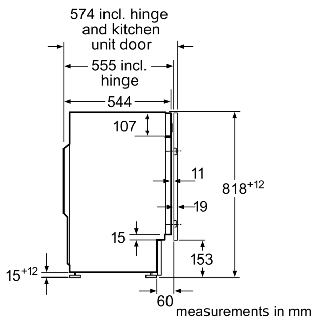
Z detail
